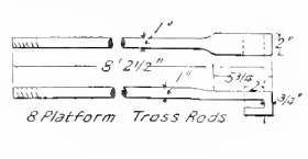
Figs. 1296-1297. Platform Truss-rod (8).
